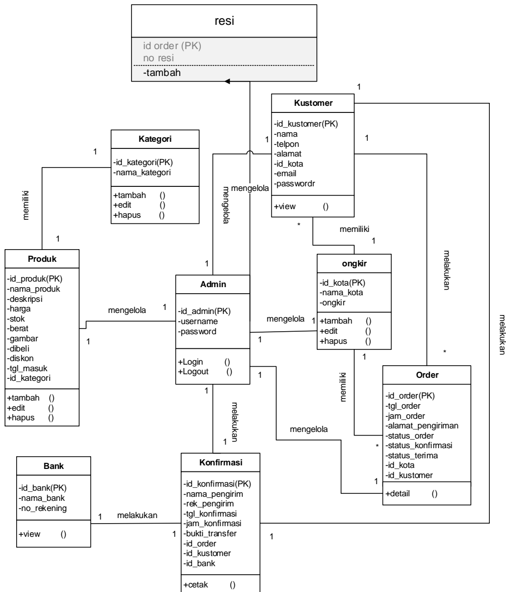
Gambar 3 Class Diagram
