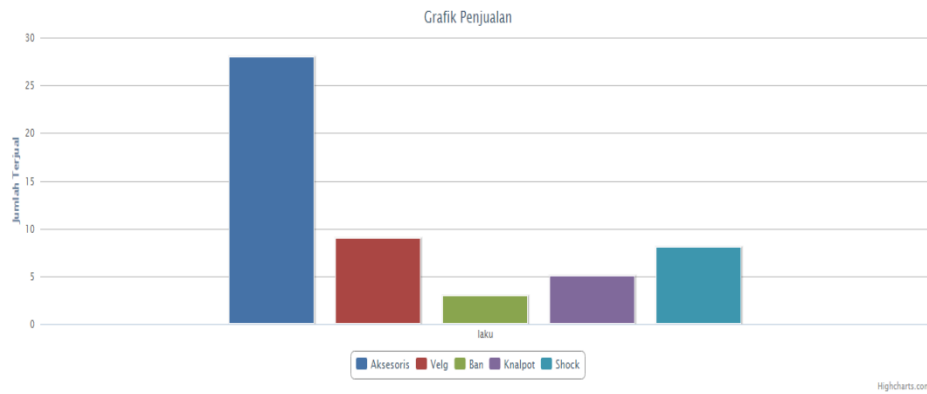
Gambar 16 Laporan Chart
